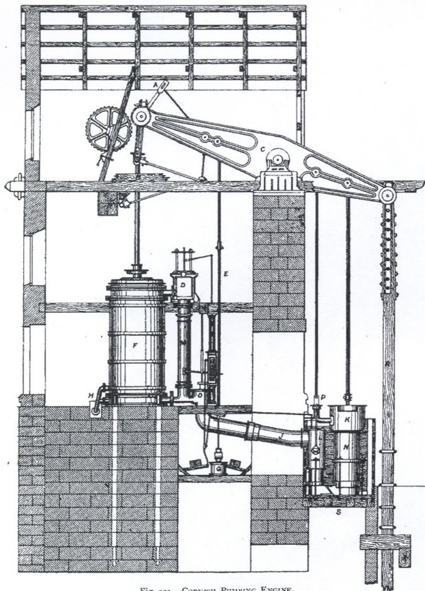
Fig. 351.—CORNISH PUMPING ENGINE.
